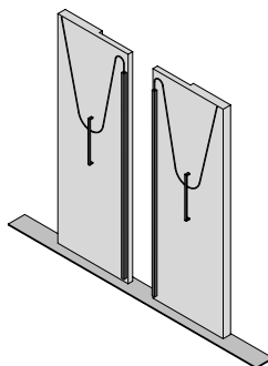
Figure 6: Dynamic mounting
